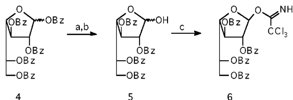
Scheme 1 a
